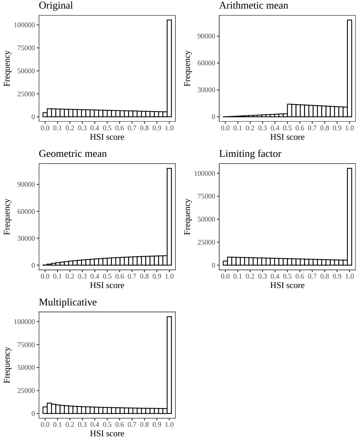
Figure 2. Empirical distributions of HSI scores for the striped bass Inland Lac Larv model using the original limiting factor model equation from Crance (1984), and an arithmetic mean, geometric mean, limiting factor, and multiplicative structure incorporating all SIV variables. Note differences in the y axis.
