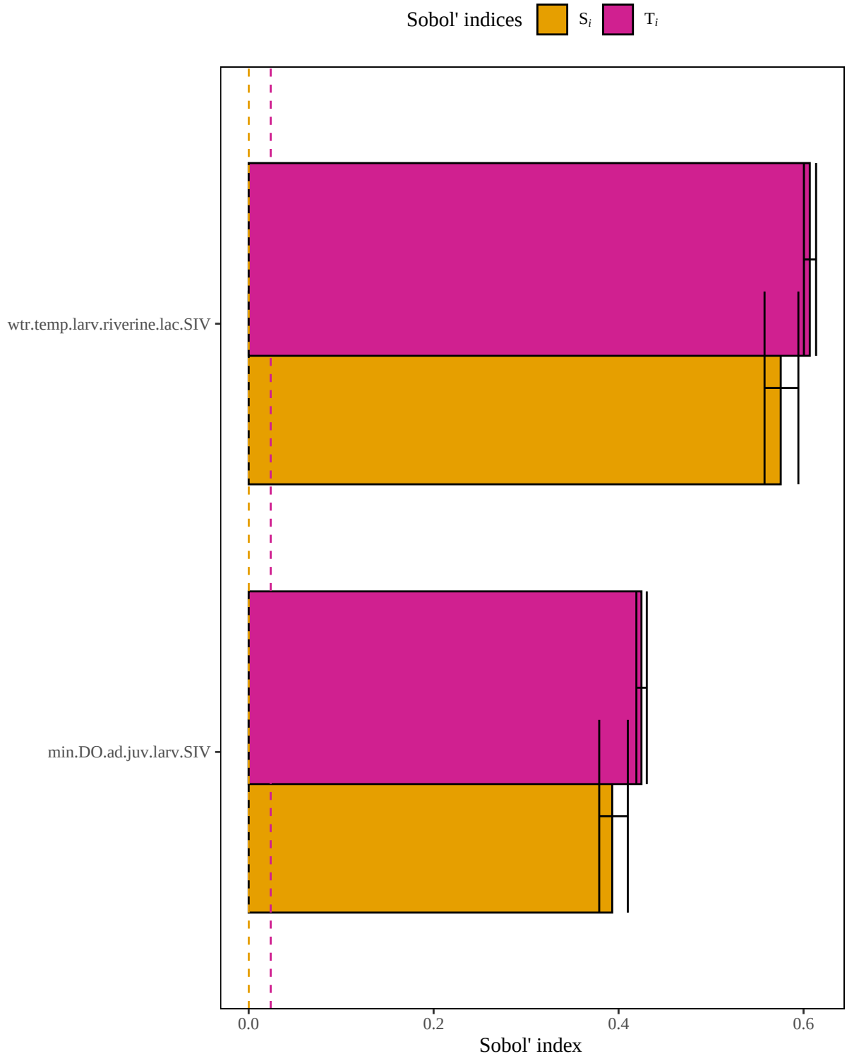
Figure 5. Results of a sensitivity analysis for the striped bass Inland Lac Larv model based on a geometric mean structure. Dashed lines represent baseline numerical approximation error for S_i and T_i ( i.e. , dummy variables).
