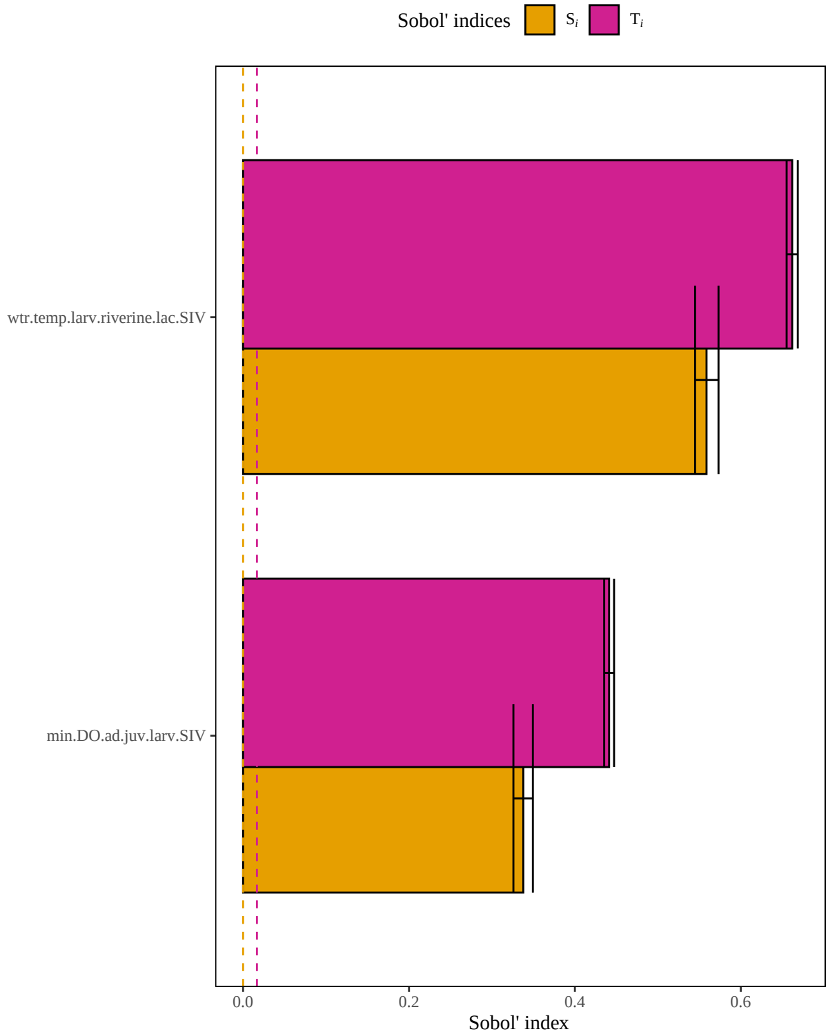
Figure 3. Results of a sensitivity analysis for the stripedbassInlandLacLarv model based on the original limiting factor model outlined in Crance (1984). Dashed lines represent baseline numerical approximation error for S_i and T_i ( i.e. , dummy variables).
